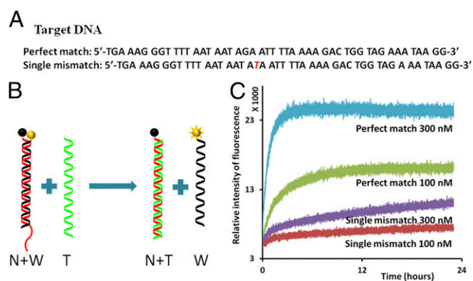
Fig. 2. Single-mismatch detection using fluorescently labeled nucleotides. (A) Sequences of the target DNA. (A, Top) Perfect match. (A, Bottom) Single mismatch. The mismatched nucleotide is marked in red. (B) Schematic of strand displacement: nucleotide with fluorophore (yellow ball) and nucleotide with quencher (black ball). Initially, the normal (N) (red) and weak (W) (black) strands are hybridized; fluorophore (yellow ball) and quencher (black ball) are adjacent so that fluorescence is quenched. When the green strand (perfect-match T) interacts with DS probe, strand displacement takes place, and the normal strand (N) and perfect-match target strand hybridize. The weak strand (W) remains single-stranded, and the fluorophore becomes active. (C) Real-time fluorescence measurement of the strand displacement. Interaction of the single-mismatch target strand with DS probe shows much less fluorescence activity than the interaction of the perfect match with DS probe. The concentration of DS probe was 10 nM, and the concentrations of T strands varied from 100 to 300 nM, shown under each plot.
